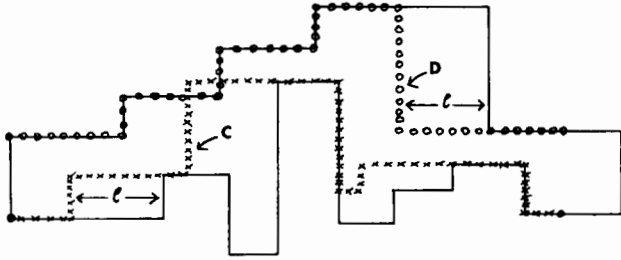
Fig. 9. The loci C and D .
