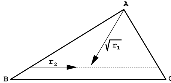
Fig. 4. Sampling a random point in a triangle.
